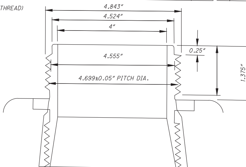
HOSE AND STEAMER NOZZLE AND CAP
