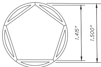
NATIONAL STANDARD PENTAGONAL OPERATING NUT
