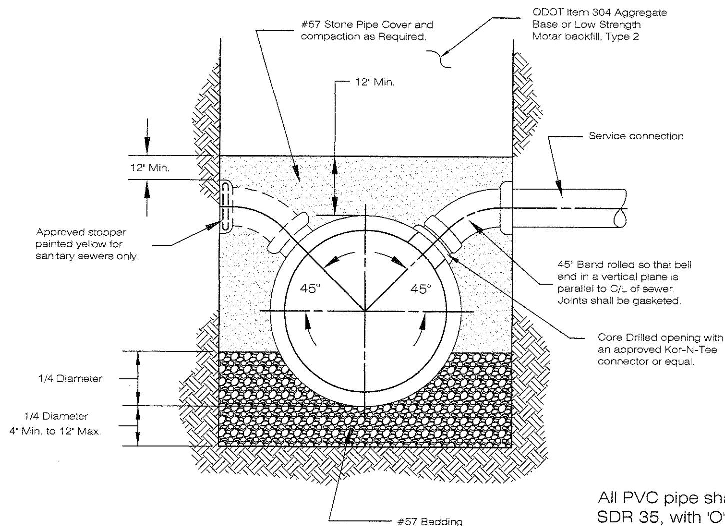
TYPICAL CORE AND TEE DETAIL (USE ON EXISTING MAINS)
